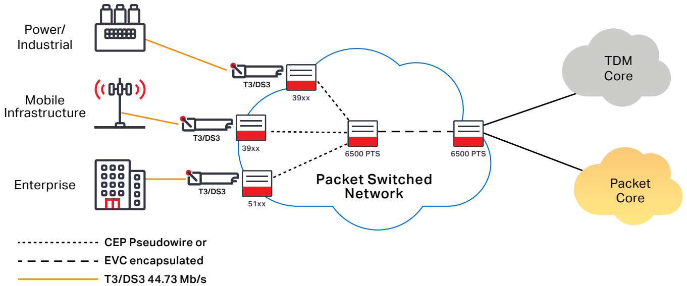
Figure 1. Aggregation of T3 to SONET/SDH
