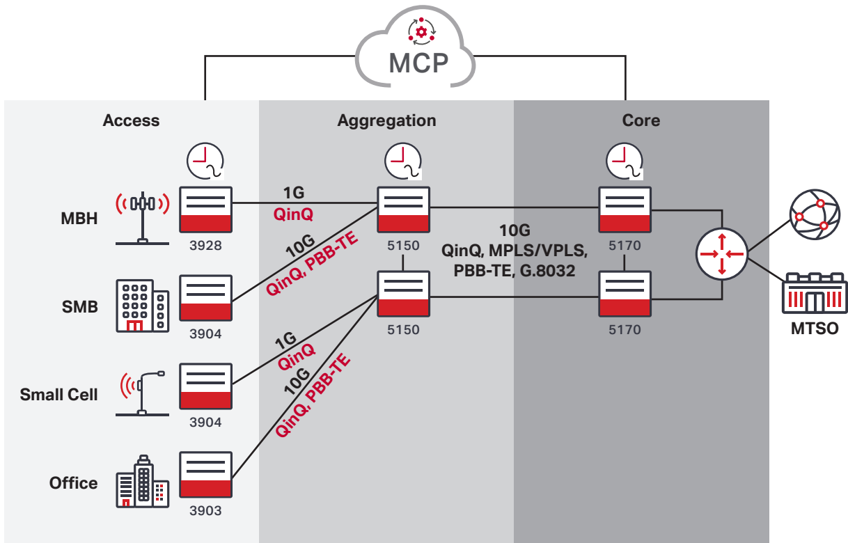
Figure 1. 5150 Ethernet aggregation
