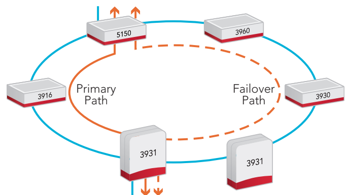
Figure 2. G.8032 ring
